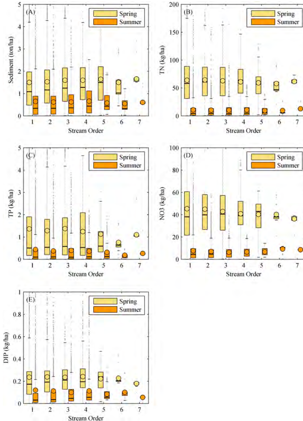
Fig. 5. Model responses for spring and summer seasons by different stream order (baseline scenario): (A) sediment; (B) total nitrogen; (C) total phosphorus; (D) \text{NO}_3 ; and (E) dissolved phosphorus.
