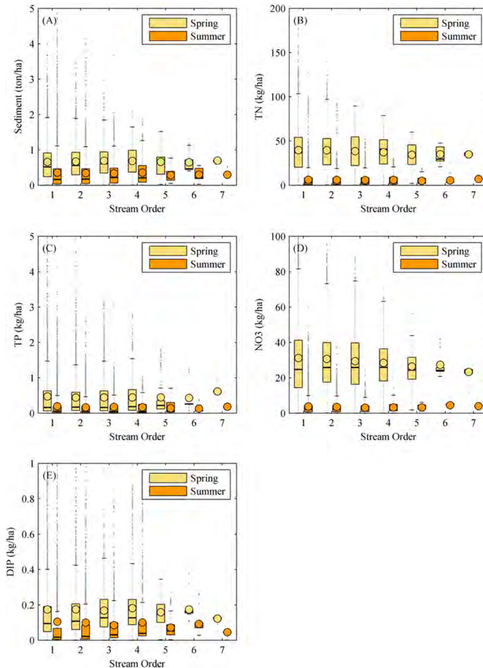
Fig. 6. Model responses for spring and summer seasons by different stream order (NM scenario): (A) sediment; (B) total nitrogen; (C) total phosphorus; (D) \text{NO}_3 ; and (E) dissolved phosphorus.
